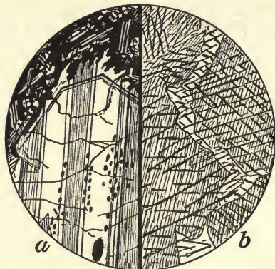
Fig. 18.— a , Plagioclase in dolerite—Tynemouth Dyke, Northumberland. \times 14 . Nicols crossed . The crystal has been enlarged by secondary outgrowths into the hemicrystalline groundmass, and the repeated twinning has been exactly reproduced. b , Hornblende in diorite—near Grands Mulets, Mt. Blanc. \times 40 . The brown crystals appear to have been shifted one against the other, and the intervening irregular areas have become filled up by colourless secondary outgrowths from one side or the other in continuity with the original crystals.
